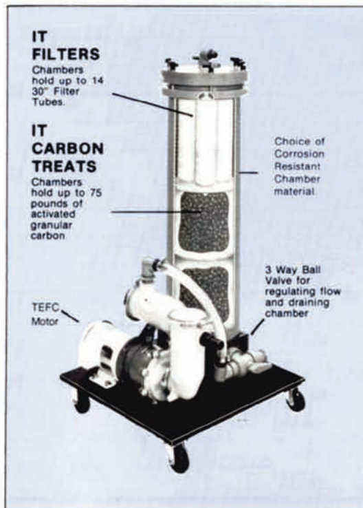
MODEL PMSFPC-3A In-Filtrator System with powerful Self-Priming, Magnetic Drive, Sealless Pump can be positioned anywhere outside tank even above it.
